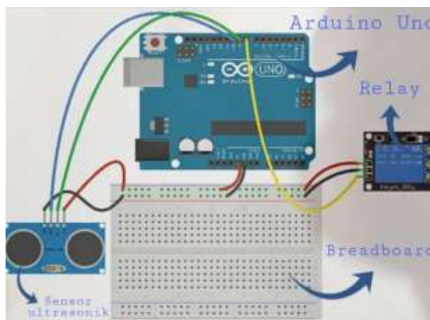
Figure 1. Ultrasonic Sensor Design Design
