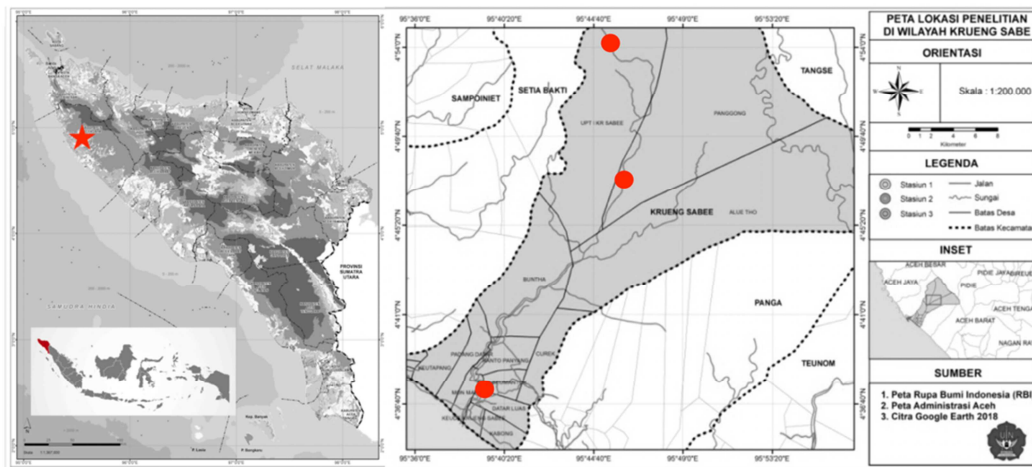
Figure 1. Map of Krueng Sabee River (red dot indicate the sampling location)
