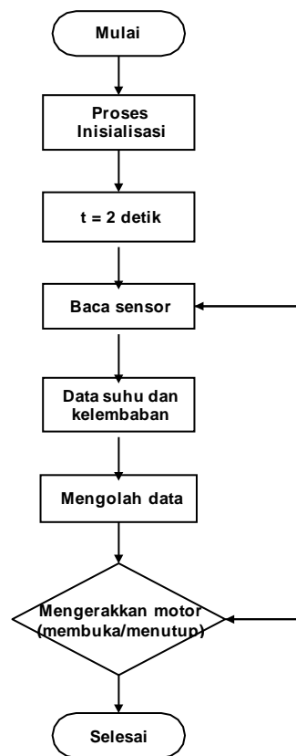
Gambar 6. Alur rancang bangun program
