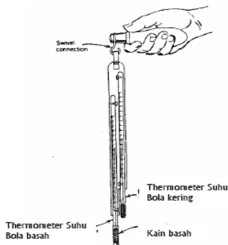
Gambar 1. Slink Psychometer . (Susanto, 2011)
